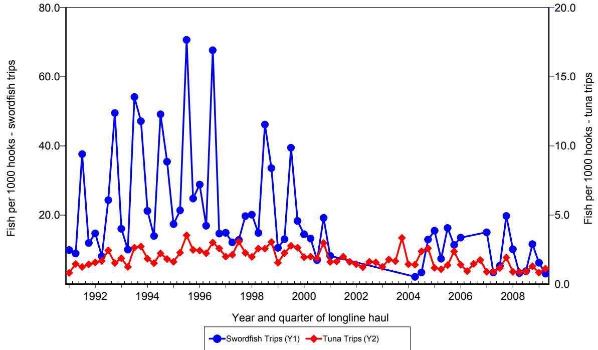
Figure 17. Quarterly CPUE of blue shark (fish per 1000 hooks) on swordfish trips and tuna trips by longline vessels based and landing in Hawaii, 1991-2009. [PIFSC IMS, Longline Logbook Data, 8/18/2009 12:47:21PM]
