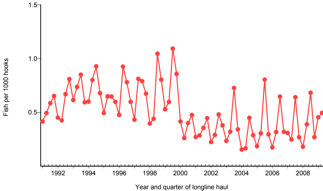
Figure 21. Quarterly CPUE of moonfish (fish per 1000 hooks) on tuna trips by longline vessels based and landing in Hawaii, 1991-2009. [PIFSC IMS, Longline Logbook Data, 8/18/2009 12:48:23PM]
