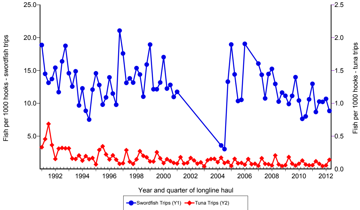
Figure 11. Quarterly CPUE of swordfish (fish per 1000 hooks) on swordfish trips and tuna trips by longline vessels based and landing in Hawaii, 1991-2012.
