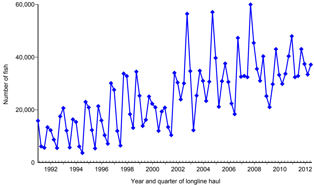
Figure 4. Quarterly catch of bigeye tuna by longline vessels based and landing in Hawaii, 1991-2012. [PIFSC IMS, Longline Logbook Data, 11/12/2012 3:03:23PM]
