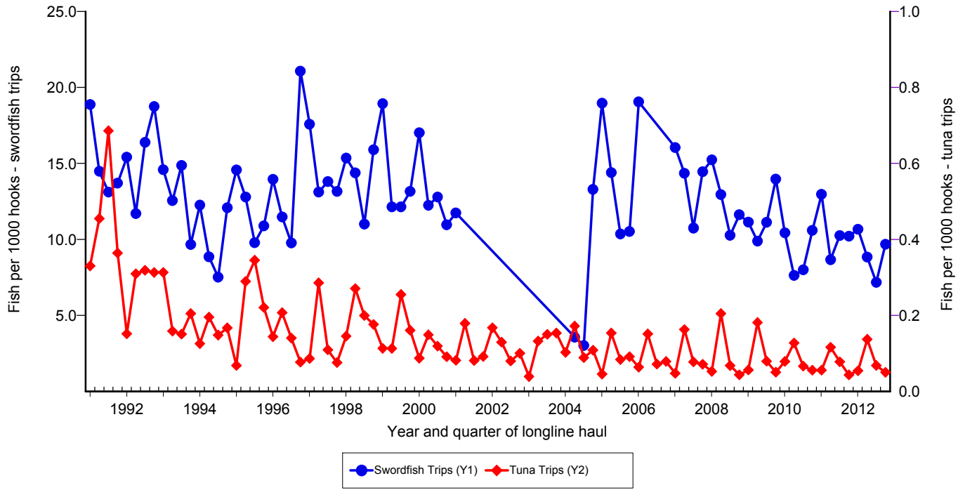
Figure 11. Quarterly CPUE of swordfish (fish per 1000 hooks) on swordfish trips and tuna trips by longline vessels based and landing in Hawaii, 1991-2012. [PIFSC IMS, Longline Logbook Data, 2/20/2013 2:35:50PM]
