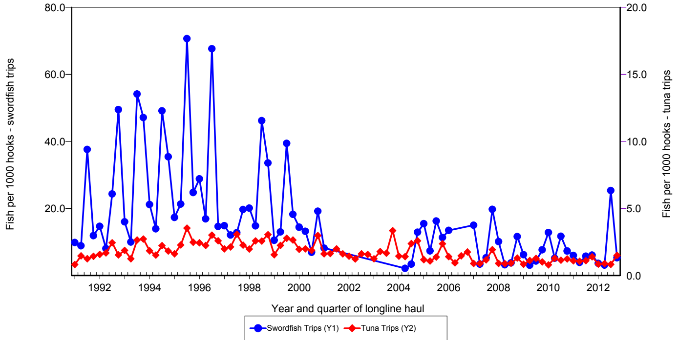
Figure 17. Quarterly CPUE of blue shark (fish per 1000 hooks) on swordfish trips and tuna trips by longline vessels based and landing in Hawaii, 1991-2012. [PIFSC IMS, Longline Logbook Data, 2/20/2013 2:37:10PM]
