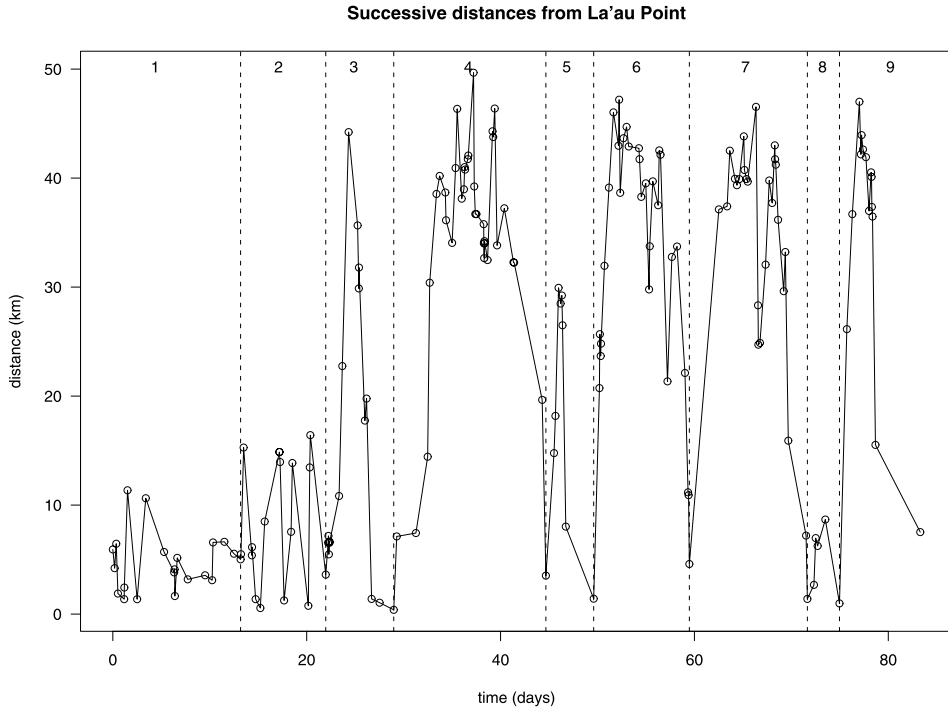
FIG 7. The distance of the seal from La'au Point plotted against the time of location. The vertical lines delineate apparent journeys.
