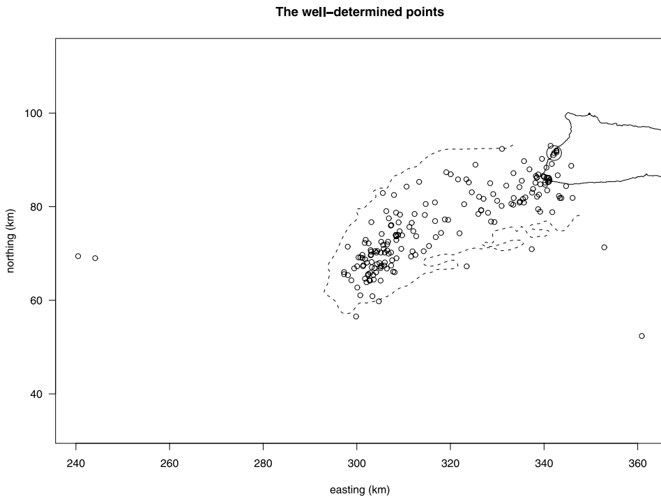
FIG 3. The figure shows the 189 well-determined locations. The dashed line is the 200 fathom line representing Penguin Bank. The large circle is the initial estimated location. There are some locations well inland suggesting the measurement error is greater than the claimed 1 km.
