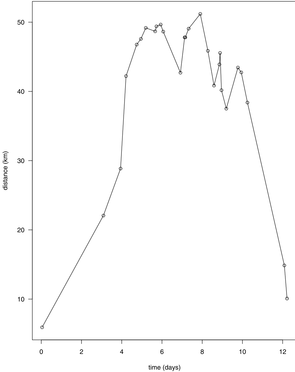
FIG 12. Distances derived from the simulation of Figure 11. The times of the points plotted are those of journey 7 of Figure 7.
