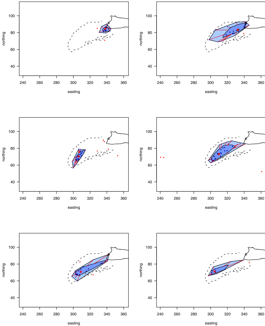
FIG 6. Bagplots of the well-determined locations for six successive 14-day periods. One reads the panels from left to right, dropping down the rows. The 200 fathom line has been added in each case.
