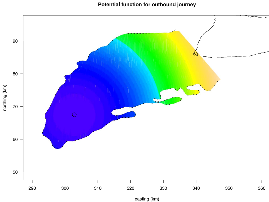
FIG 9. The potential function employed to describe the outbound and foraging journeys. The circle in the SW corner represents an assumed point of destination. Lighter values correspond to large and darker to smaller potential function values. The seal is attracted to the darker region.
