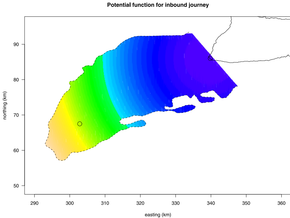
FIG 10. The potential function employed to describe the inbound journey. The circle on Molokai represents La'au Point. Again the animal is pulled towards the darker region.
