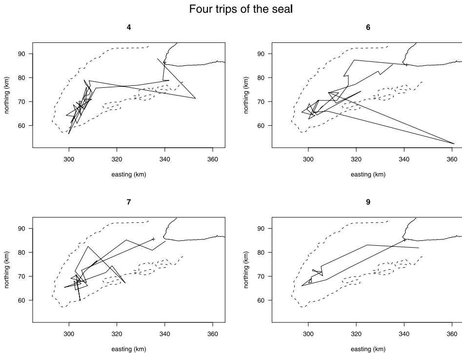
FIG 8. The separate plots display the journeys 4, 6, 7, and 9 delineated in Figure 7. The initial point of a trip is indicated by “+”.
