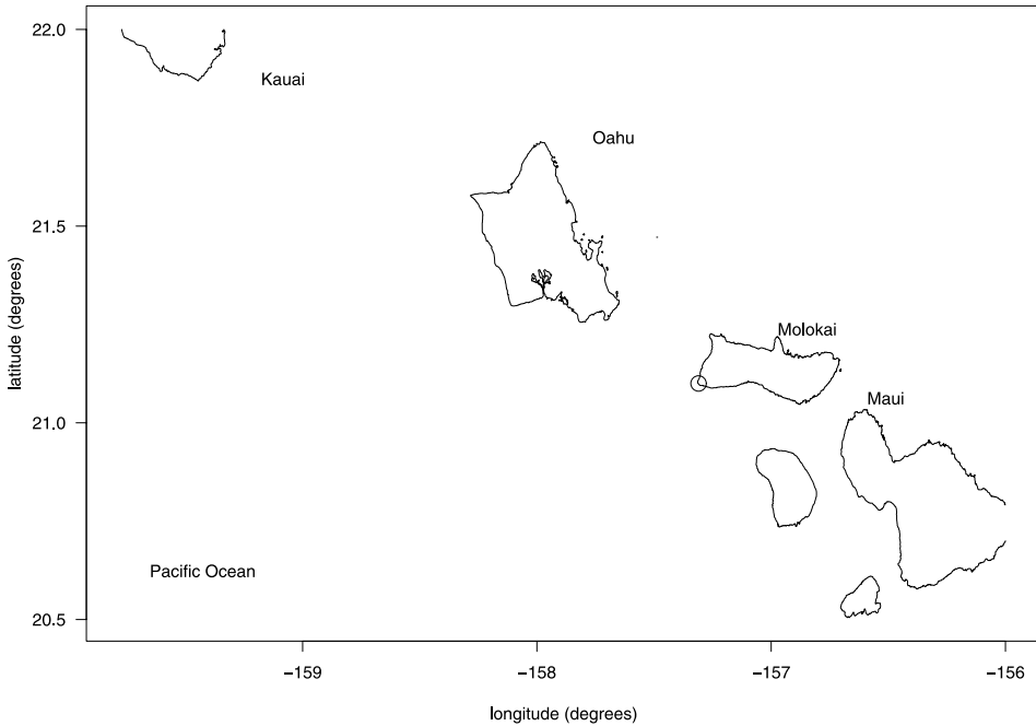
FIG 1. The central Hawaiian Islands. The circle on the southwest corner of Molokai is La'au Point, the location where the seal was initially captured.
