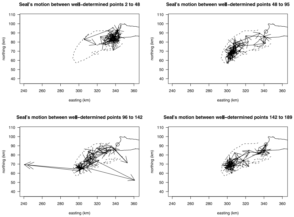
FIG 4. Directed arrows representing the motion in four contiguous segments. The data employed are the well-determined locations. The track starts at the large circle.
