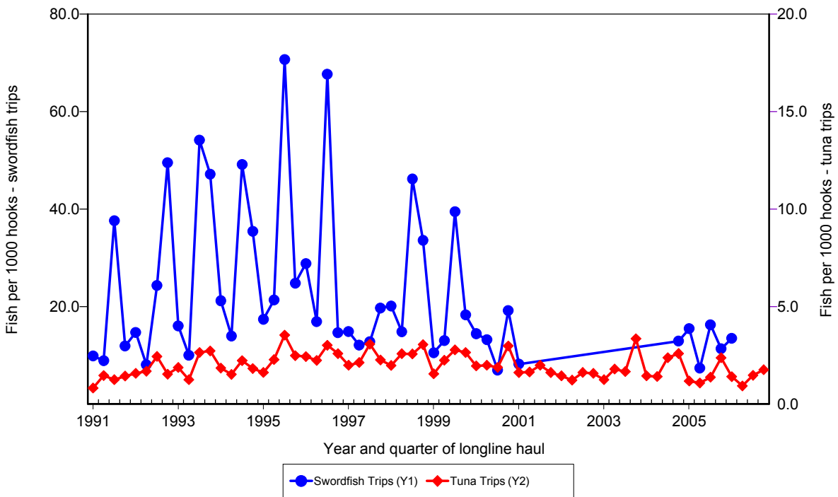
Figure 17. Quarterly CPUE of blue shark (fish per 1000 hooks) on swordfish trips and tuna trips by longline vessels based and landing in Hawaii, 1991-2006. [PIFSC IMS, Longline Logbook Data, 2/16/2007 9:41:26AM]
