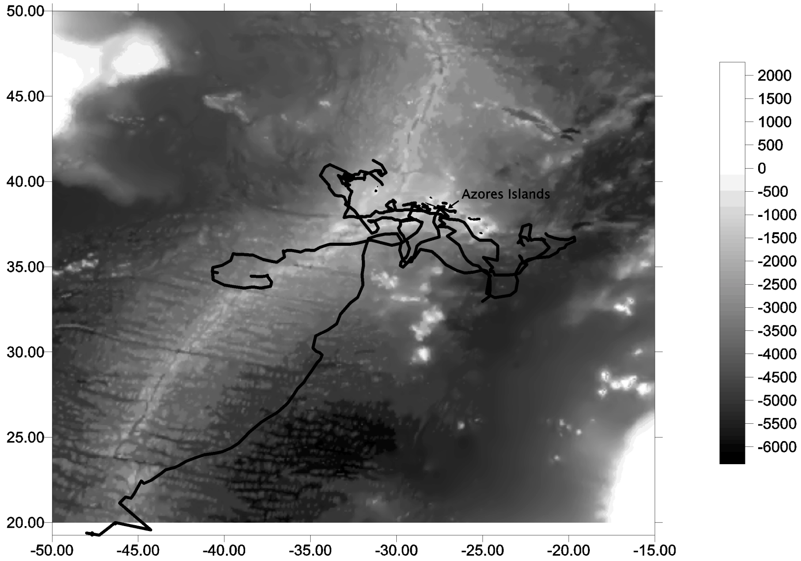
Figure 2. Movements of all turtles with respect to bathymetry. Depth scale is in meters.
