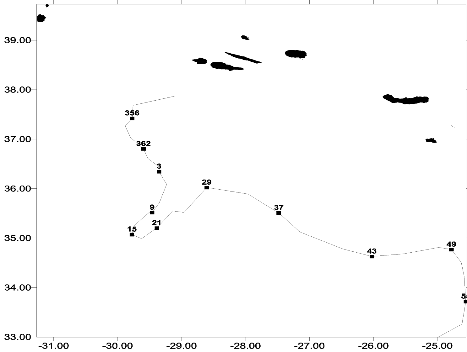
Figure 1(h). Movements of turtle 23659 from release on 12-5-98 (day of year 339) through 2-28-99 (day of year 59).
