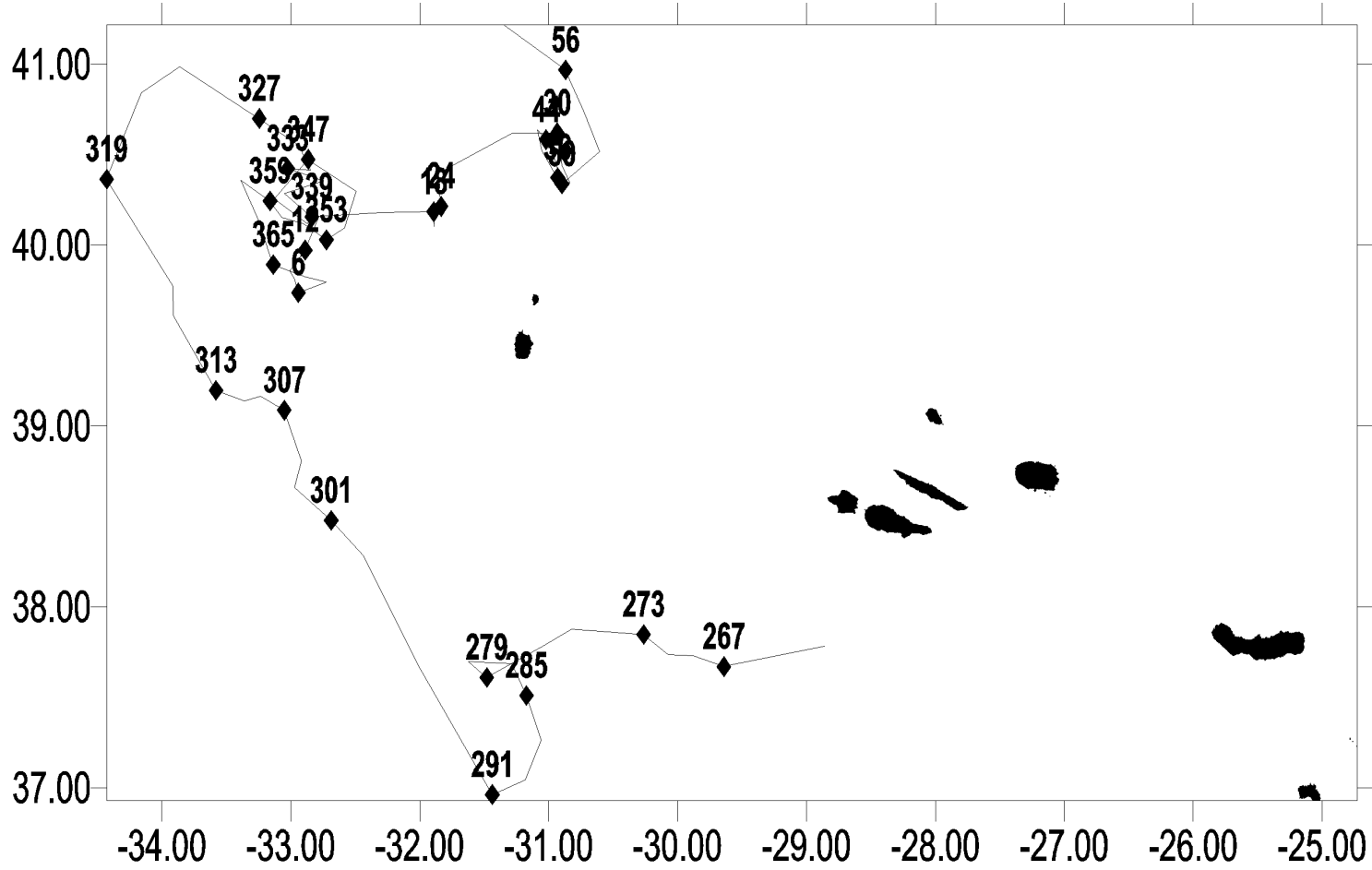
Figure 1(c). Movements of turtle 23660 from release on 9-17-98 (day of year 261) through 2-28-99 (day of year 59).
