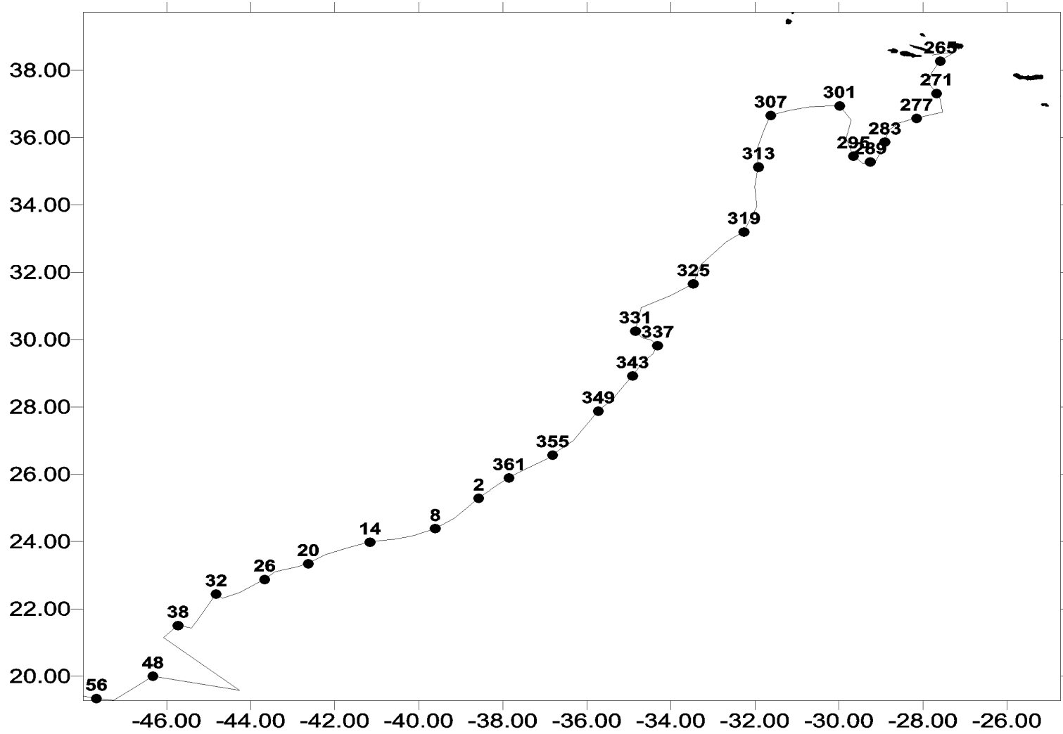
Figure 1(b). Movements of turtle 23662 from release on 9-15-98 (day of year 259) through 2-28-99 (day of year 59).
