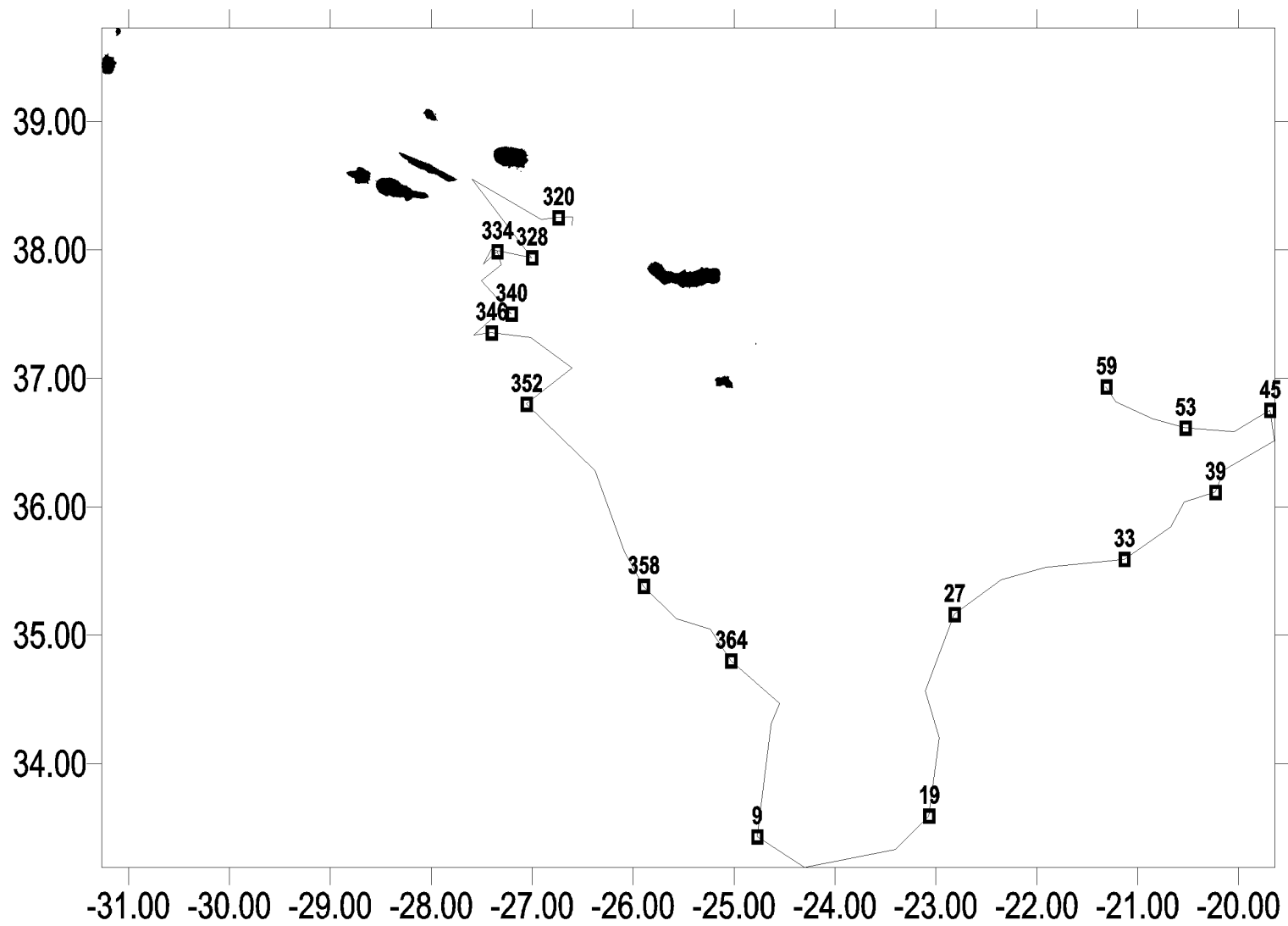
Figure 1(g). Movements of turtle 22530 from release on 11-11-98 (day of year 316) through 2-28-99 (day of year 59).
