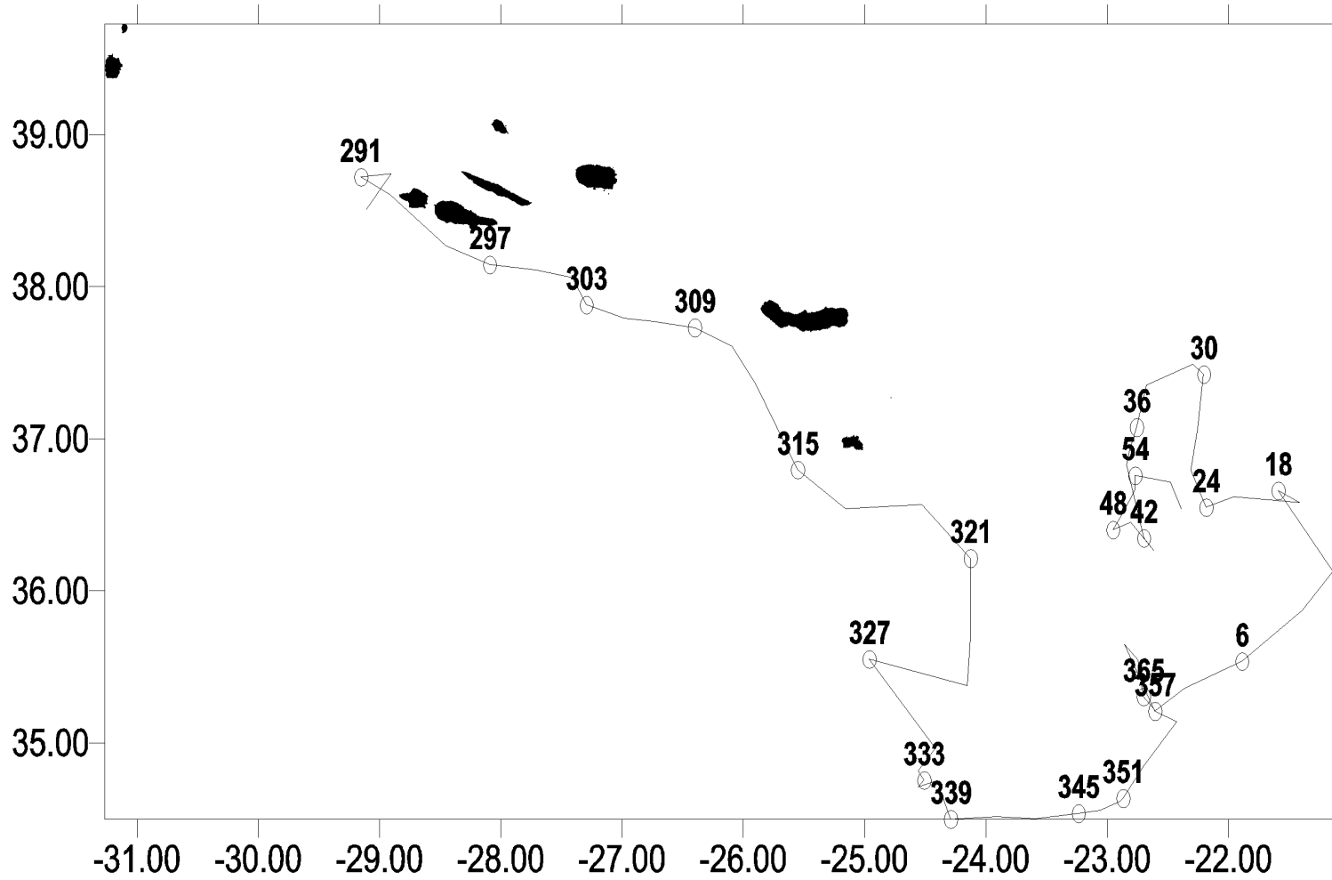
Figure 1(e). Movements of turtle 23661 from release on 10-12-98 (day of year 286) through 2-28-99 (day of year 59).
