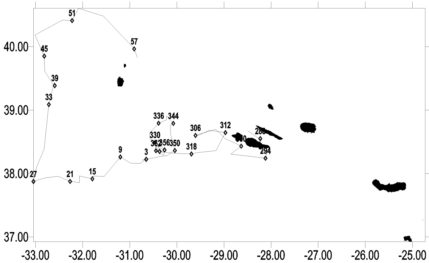
Figure 1(d). Movements of turtle 23658 from release on 10-7-98 (day of year 281) through 2-28-99 (day of year 59).
